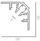
Track T InCorner
