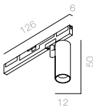
SPS Locus 0230 36° PB DIM
