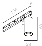
SPS Locus Super Spot 0427 6° BK DIM
