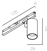
SPS Locus 0430 36° PB DIM DALI
